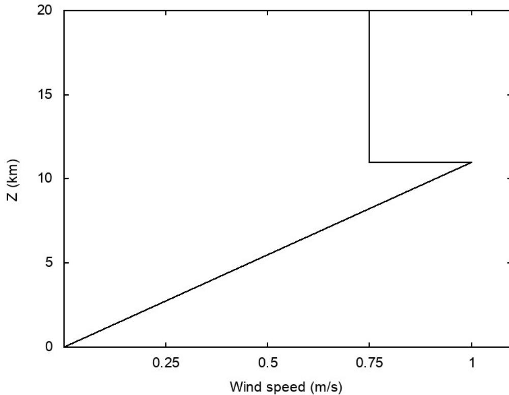
Figure 1: Wind profile generated by PARFIT.
