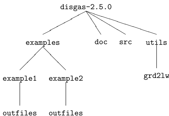
Figure 2: Directory tree of disgas-2.5.0 .
